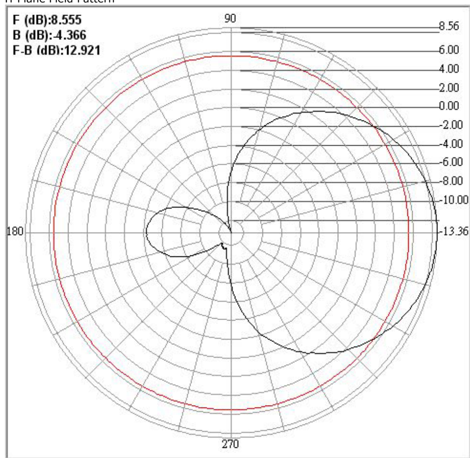
H-Plane Field Pattern
