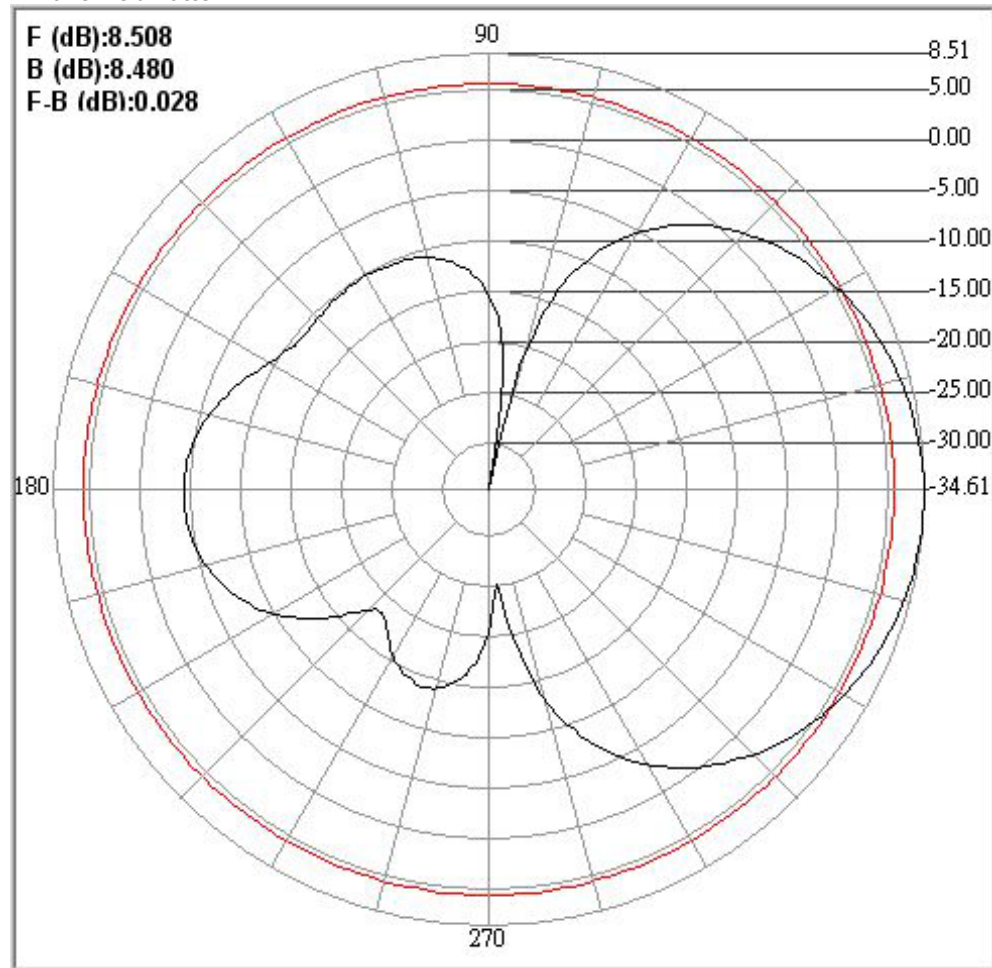
E-Plane Field Pattern
