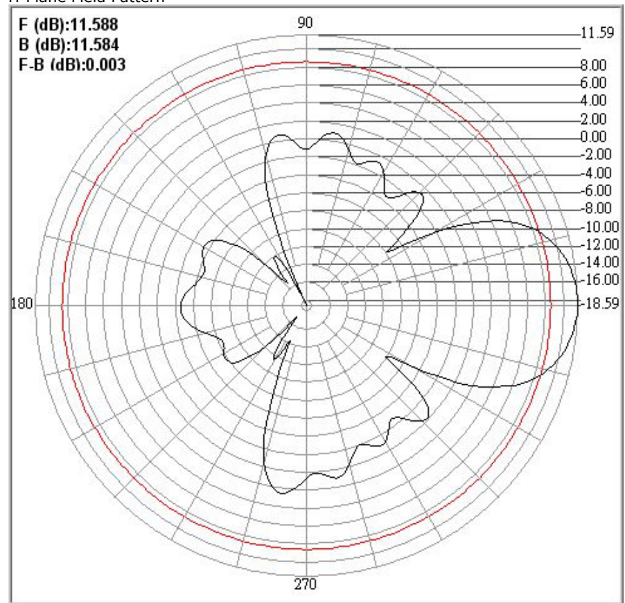
H-Plane Field Pattern
