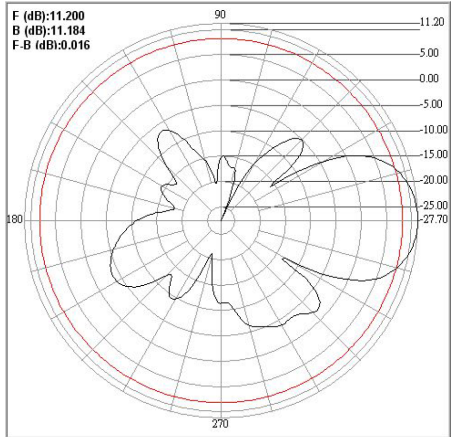
E-Plane Field Pattern
