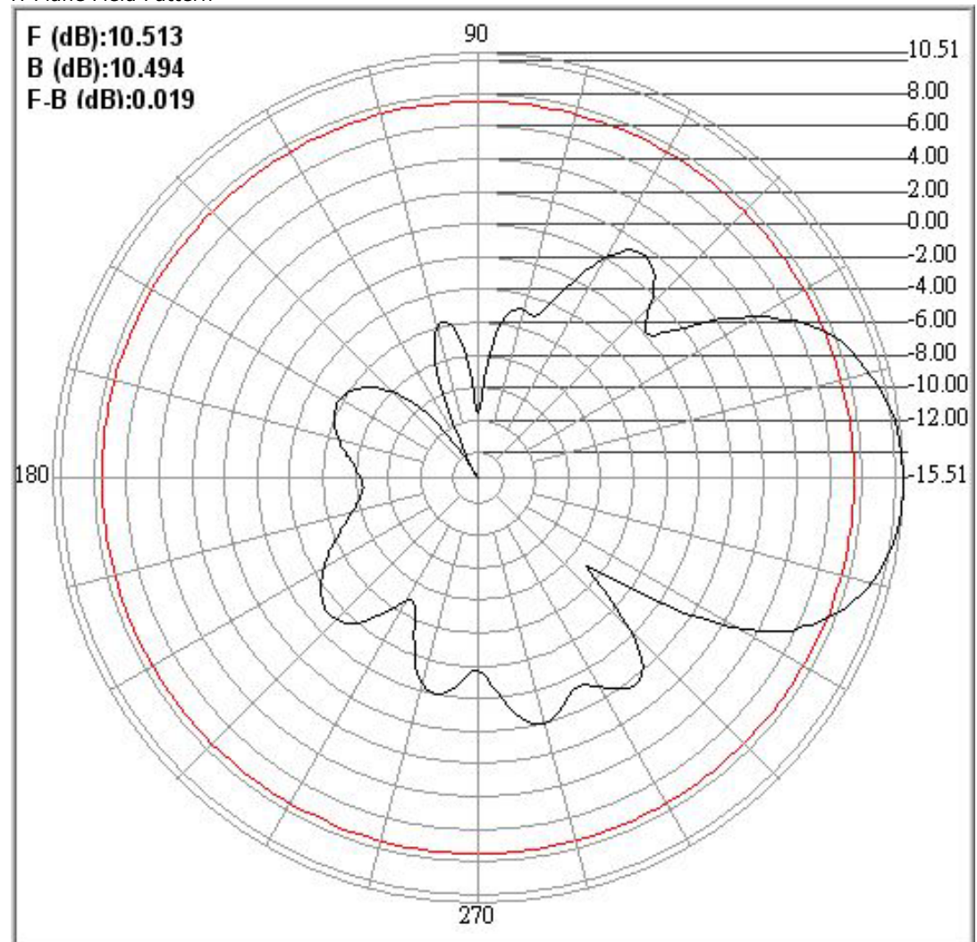
H-Plane Field Pattern
