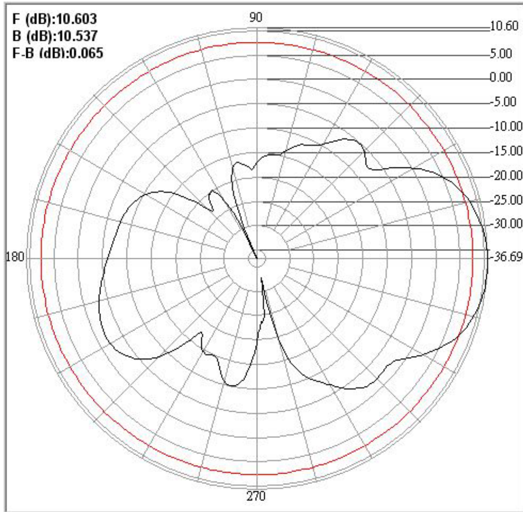
E-Plane Field Pattern
